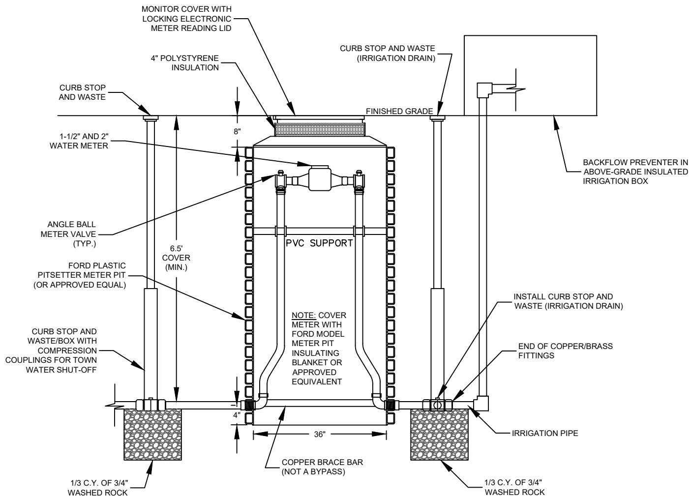
IRRIGATION METER PIT DETAIL
