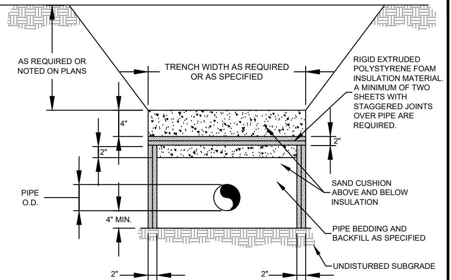
NARROW TRENCH INSULATION DETAIL
