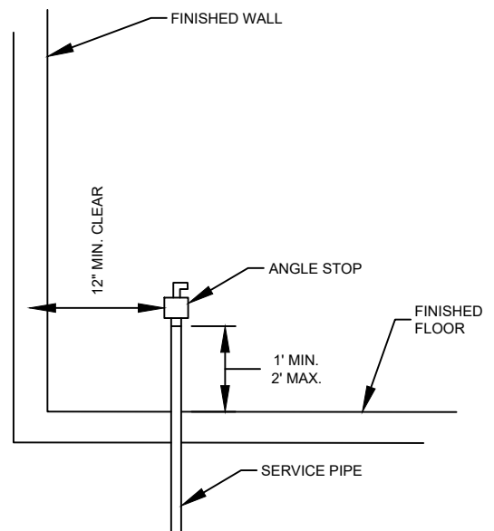
1-1/2 " AND 2" COPPER SERVICES PROFILE VIEW
