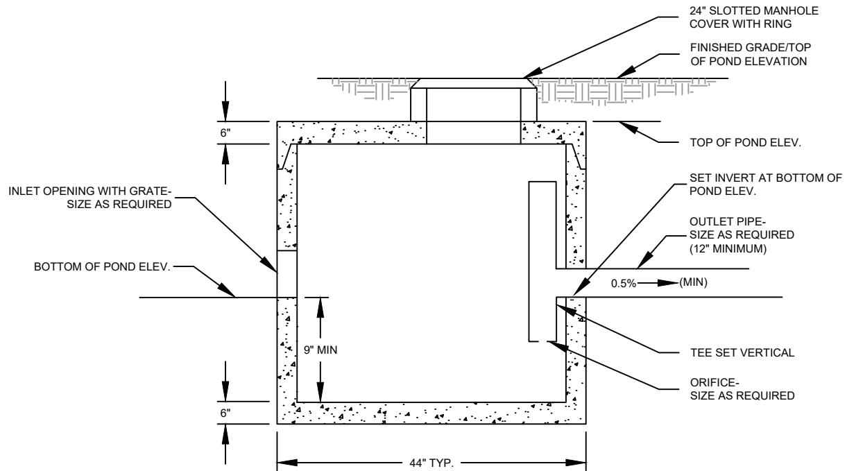
SIDE VIEW
