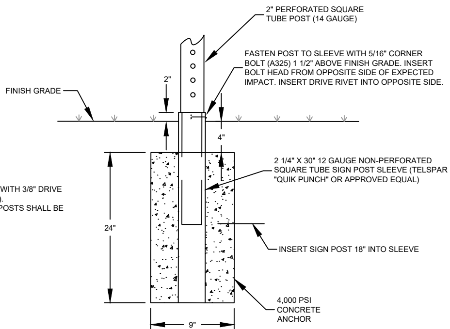
SIGN POST FOUNDATION DETAIL
