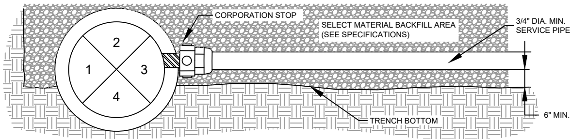
DETAIL OF A PROPERLY INSTALLED CORPORATION STOP
