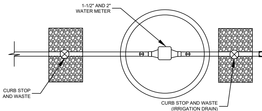
IRRIGATION METER PIT DETAIL - PLAN VIEW
