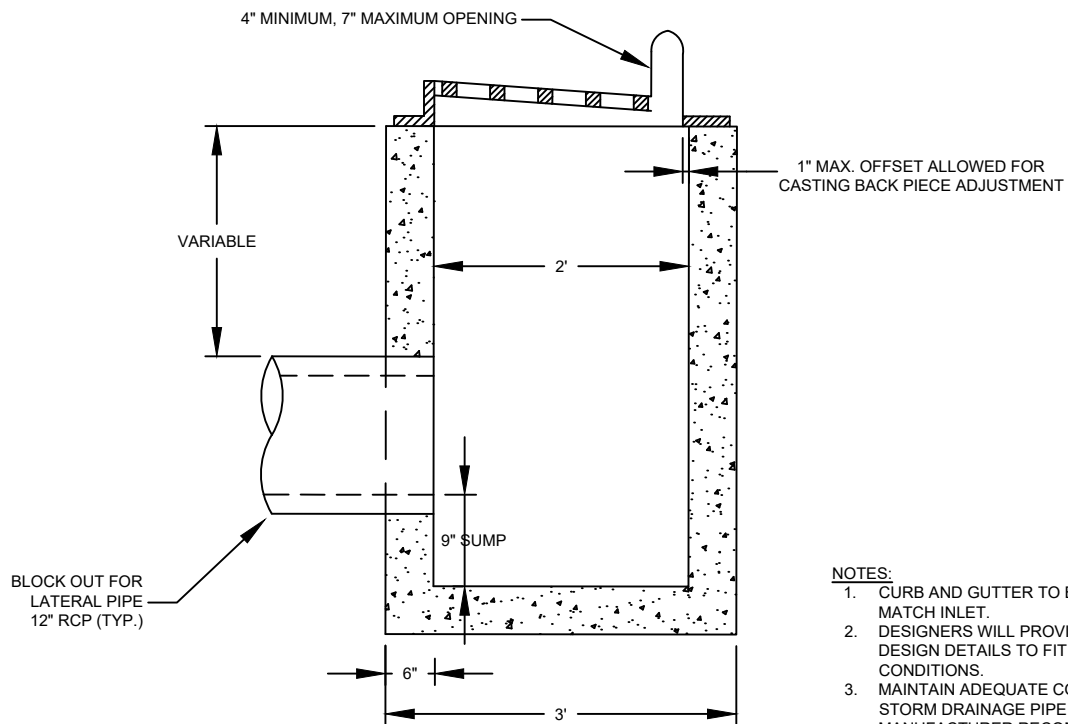
FRONT VIEW
