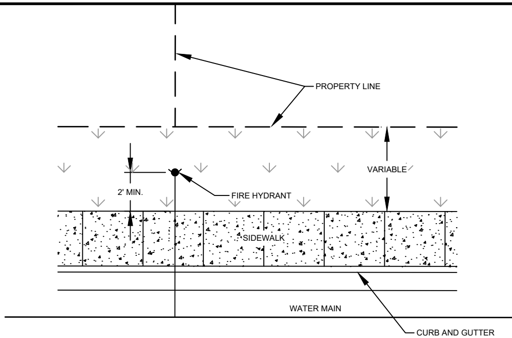
CURB WALK DETAIL
