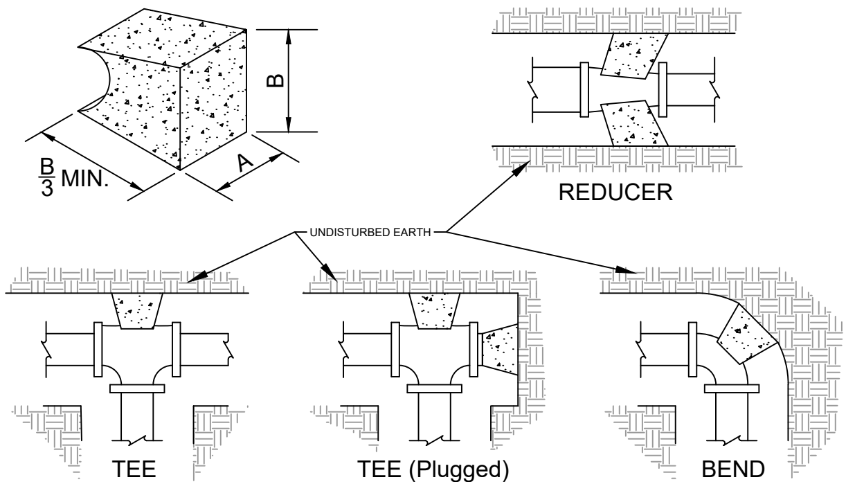
STANDARD DIMENSIONS FOR THRUST BLOCKING
