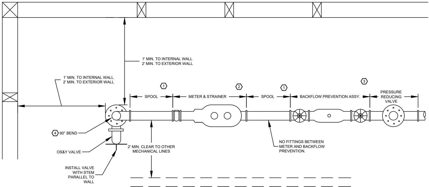
PLAN VIEW
