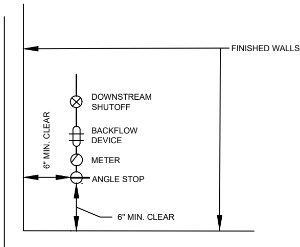
3/4" AND 1" COPPER SERVICES PLAN VIEW
