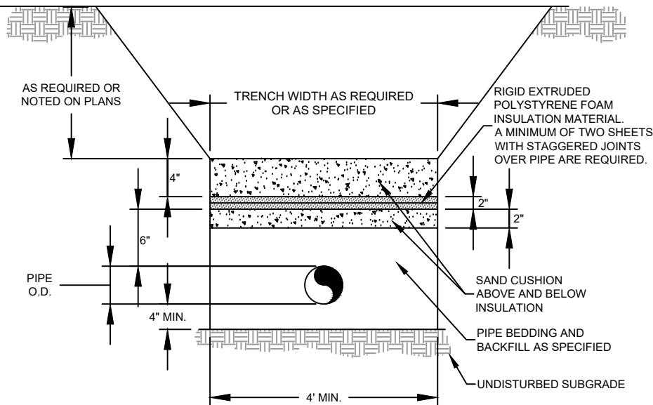
TYPICAL INSULATION DETAIL
