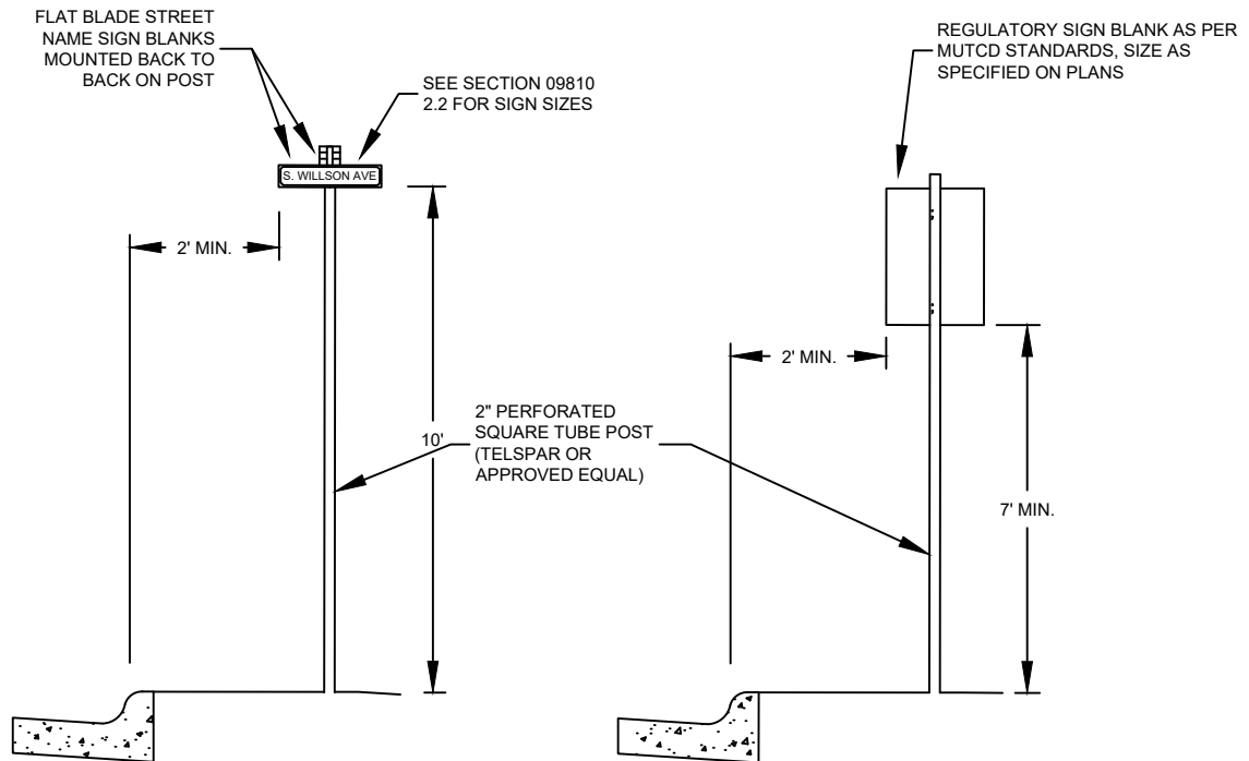
STREET MARKER SIGN
